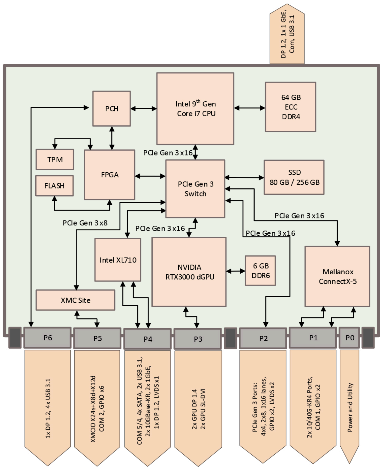
Block diagram (Non-SOSA)
