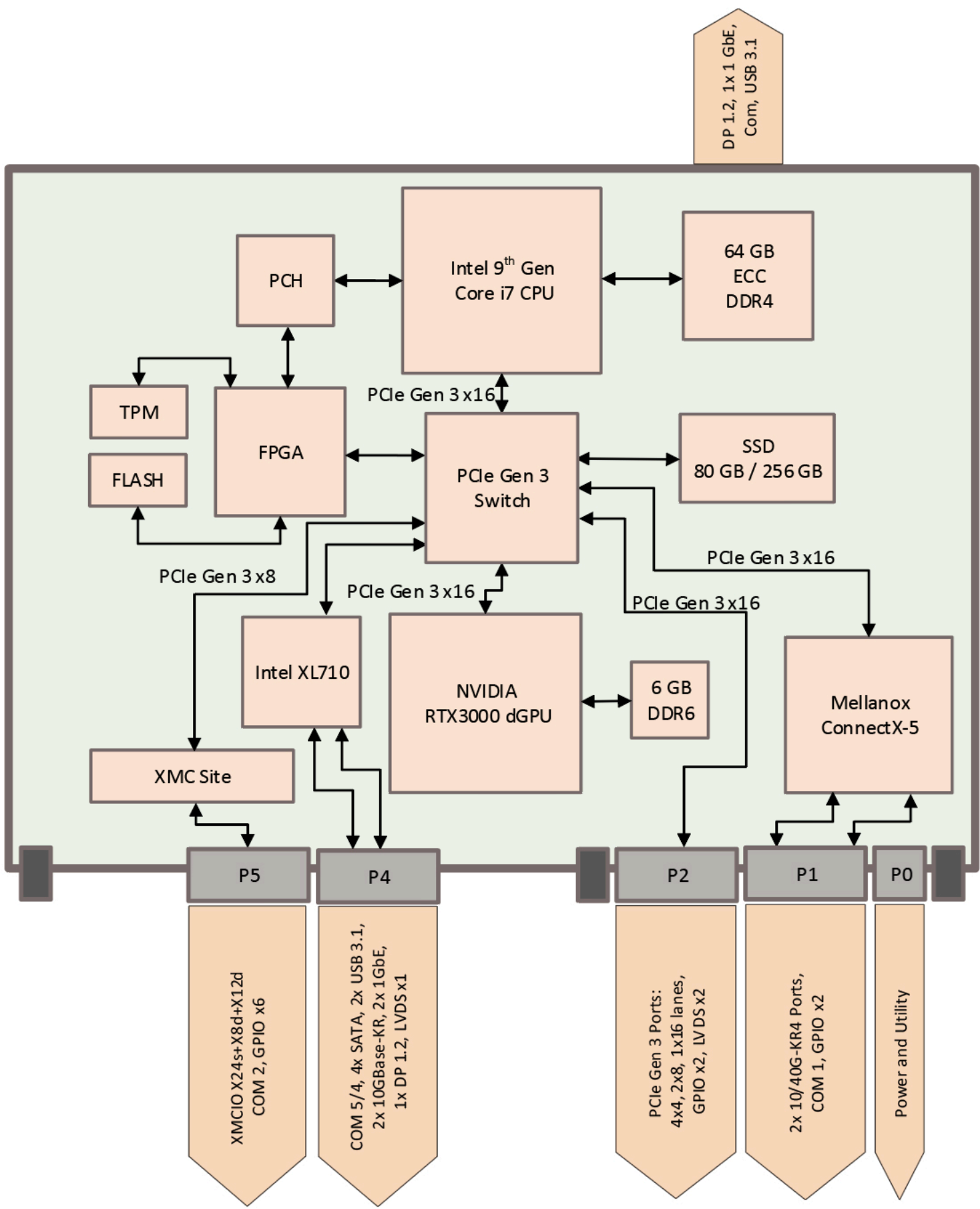
Block diagram (SOSA-Aligned)
