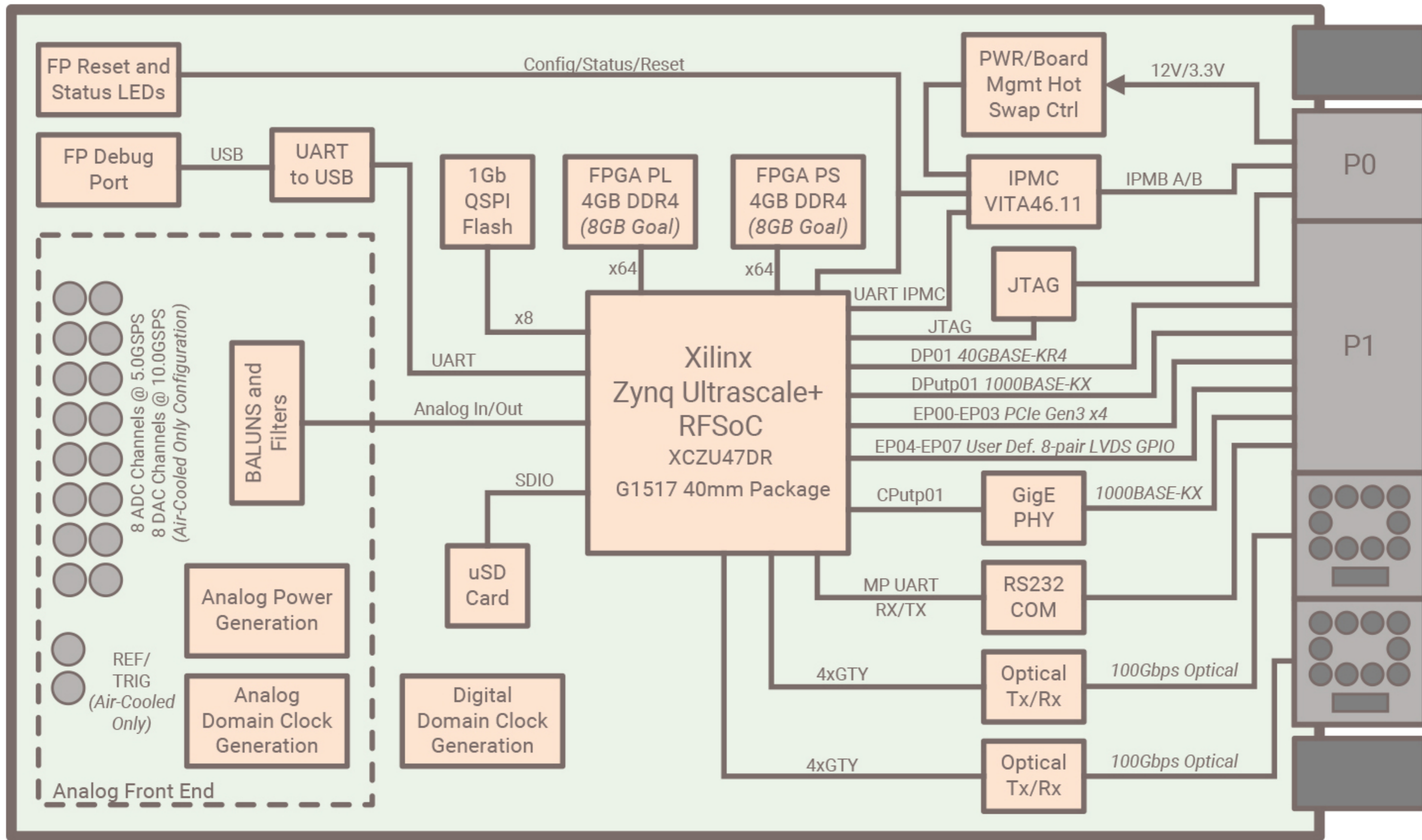
Block diagram intended as a reference for basic features and connections and not an actual product layout or design.
