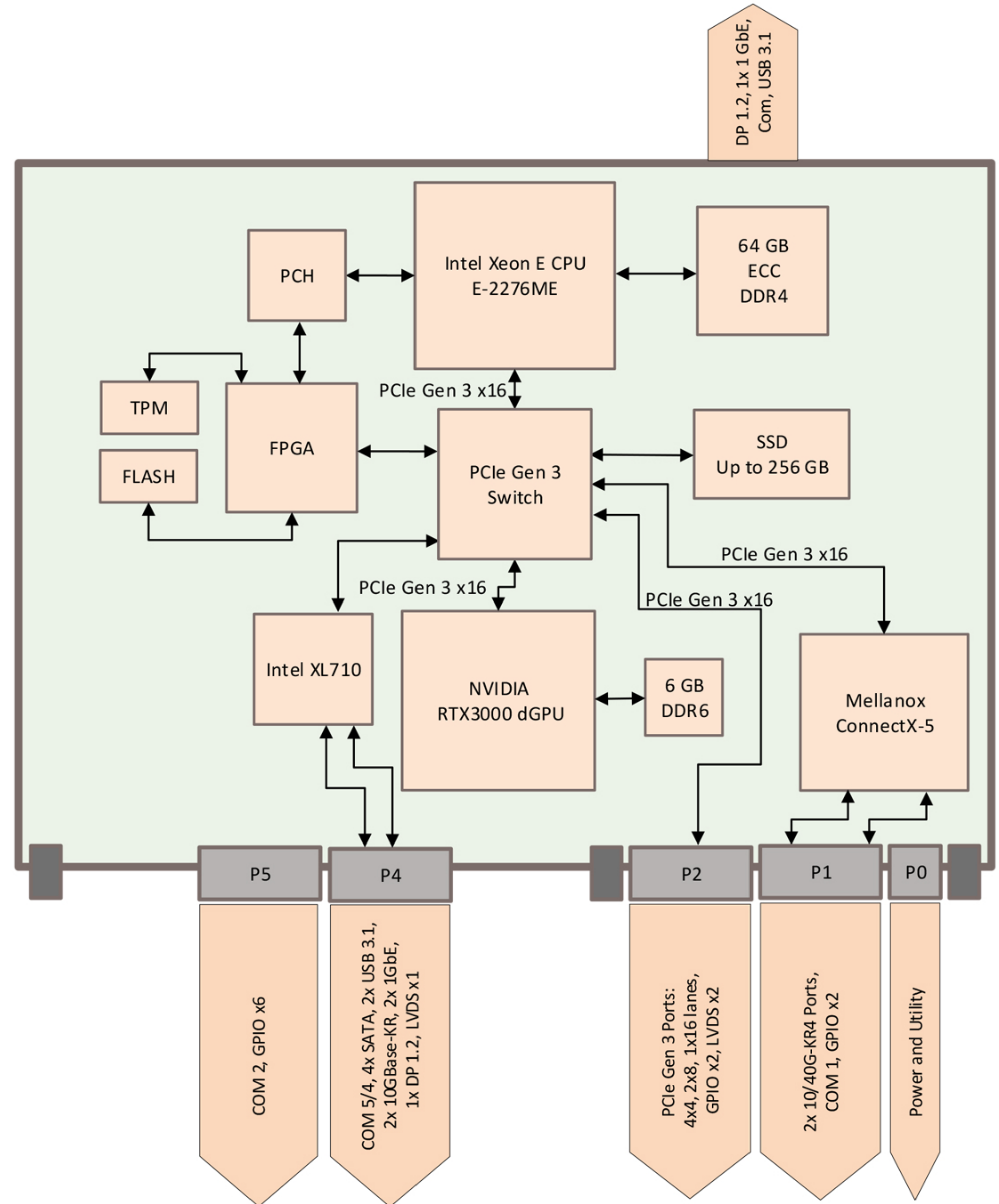
Block diagram (SOSA-Aligned)
